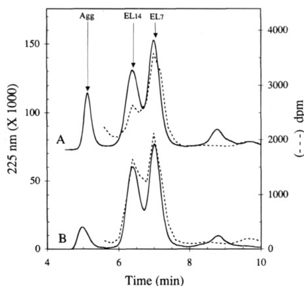
FIGURE 6: Titration of acid denatured [ 35 S]Rubisco binding. An equal mass of Tbr -EL 14 • Tbr -ES 7 and Tbr -EL 7 (A) or an equal mass of Eco -EL 14 and Tbr -EL 7 (B) was challenged with a 2–3-fold excess of acid-denatured Rubisco (see Experimental Procedures). Absorbance at 225 nm (solid lines) and dpm (dashed lines) (top data displaced upward by 0.075 and 1900 dpm, respectively) demonstrate twice as much Rubisco bound to doubly toroidal Eco -EL 14 as bound to Tbr -EL 14 • Tbr -ES 7 on a molar basis. Note that with an excess of Rubisco over GroEL binding sites, a large peak of aggregates elutes at 5 min.
